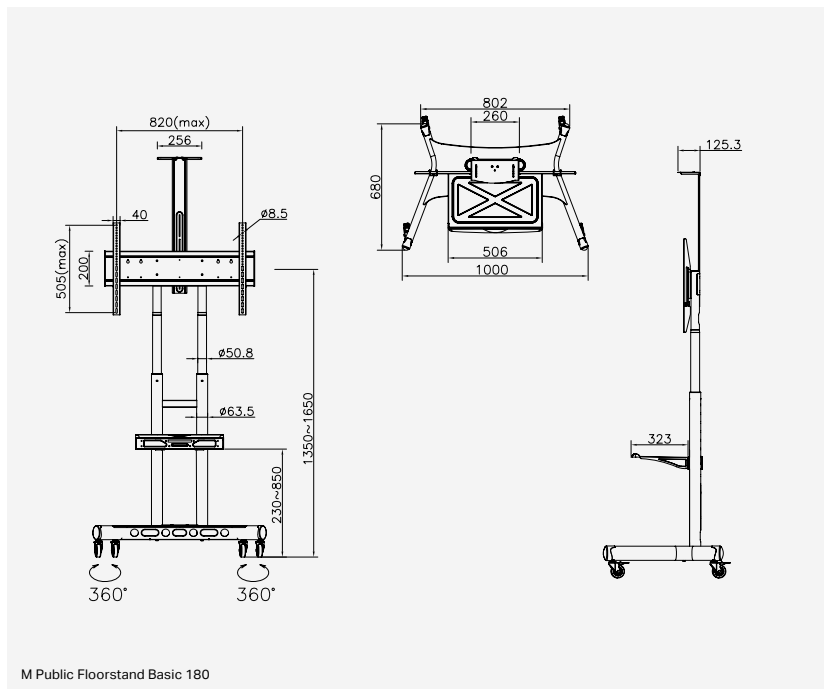
M Public Floorstand Basic 180
