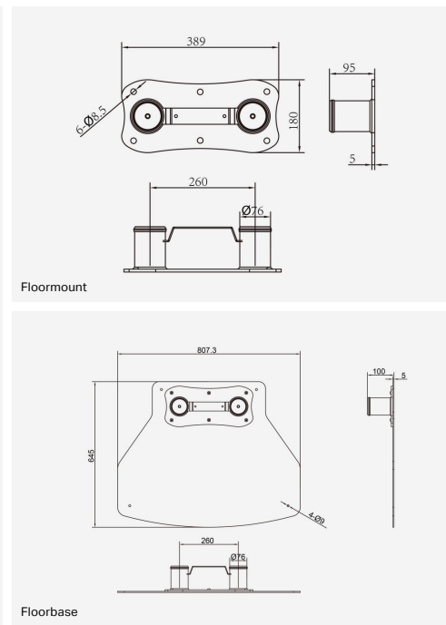
Floorbase
