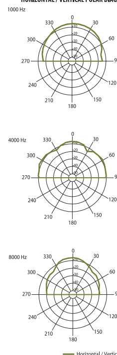
HORIZONTAL / VERTICAL POLAR DIAGRAMS
