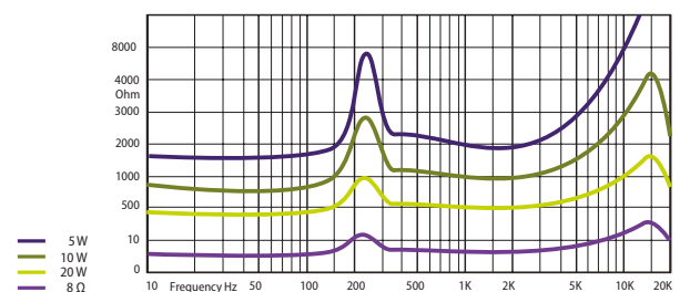
IMPEDANCE
